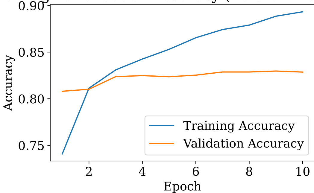
Training vs Validation Accuracy (Before Fine-Tuning)
